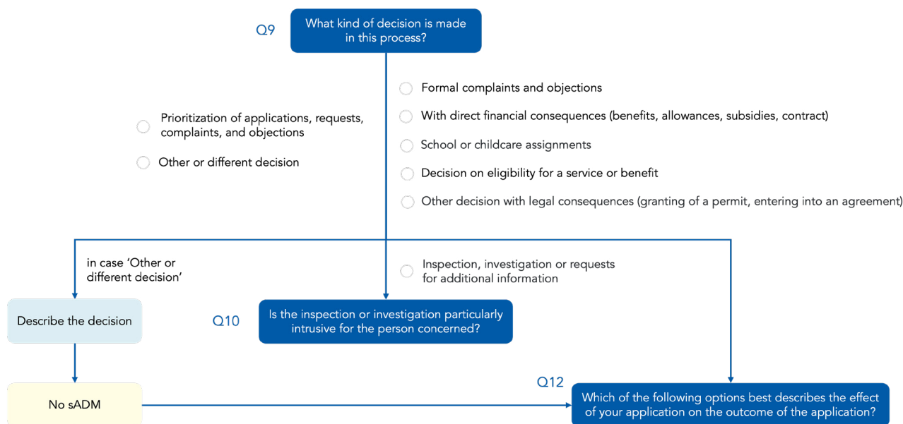
Figure 14 - Q9 of the questionnaire Identification, determines what type of decision is made in the process the algorithmic application is used in.
