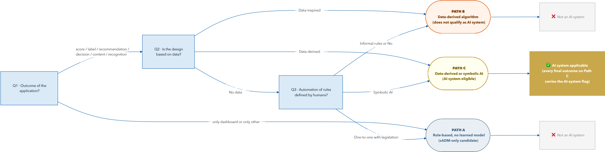
Figure 6 - Flowchart determining whether an AI system is applicable or not.
