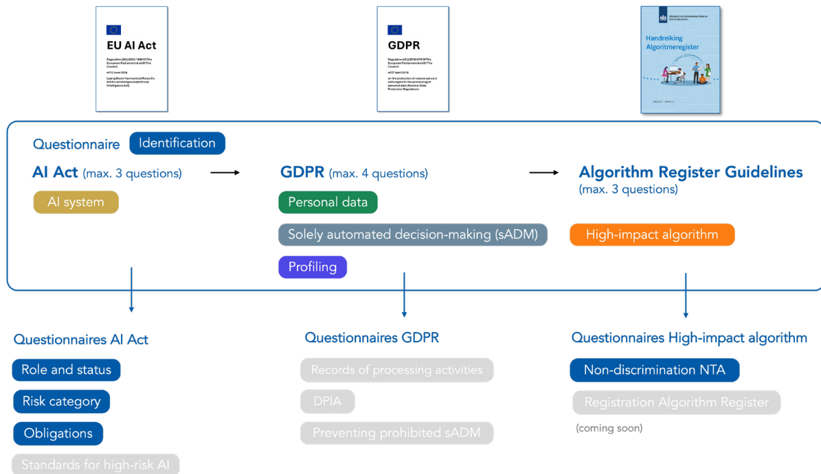
Figure 1 - Overview of the flow of dynamic questionnaires in the AI AQT. Responses to earlier questions are taken into account in order to minimize the number of questions presented to the user.
