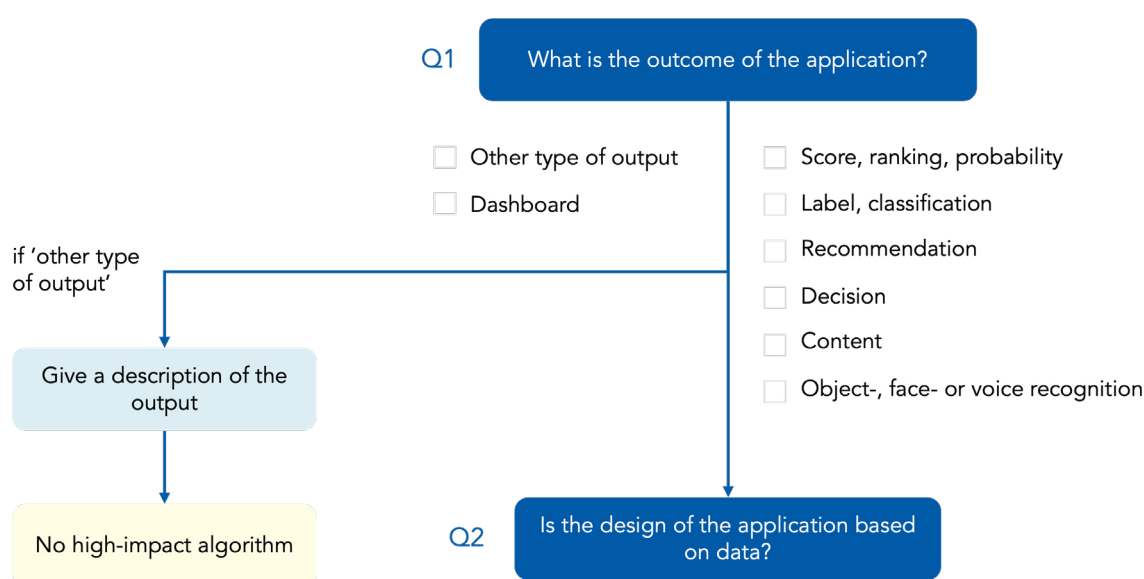
Figure 19 - Q1 of questionnaire Identification concludes that the application does not qualify as a high-impact algorithm if a ‘Dashboard’ or ‘Other type of output’ is at stake.
